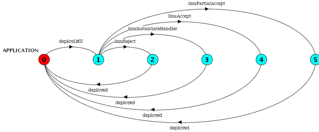
Figure 3.16: A state machine representing an application receiving an LMU.
